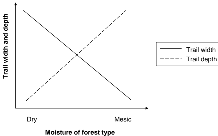
Fig. 5. Schematic presentation on the dependence of trail widths and depths on the moisture conditions (dry to mesic) after recreational use (hiking and horse riding). In reality, relationships are not linear.
